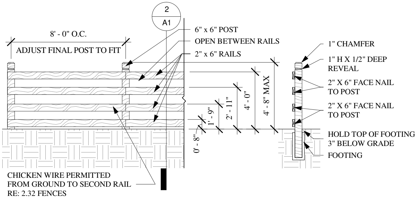
LOT BOUNDARY SPLIT RAIL FENCE ELEVATION
