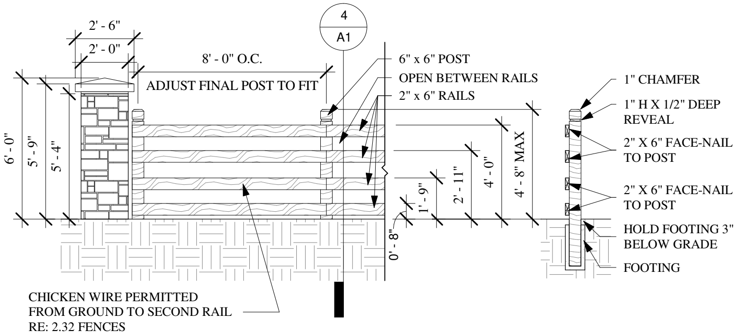
OPEN SPACE SPLIT RAIL FENCE ELEVATION
